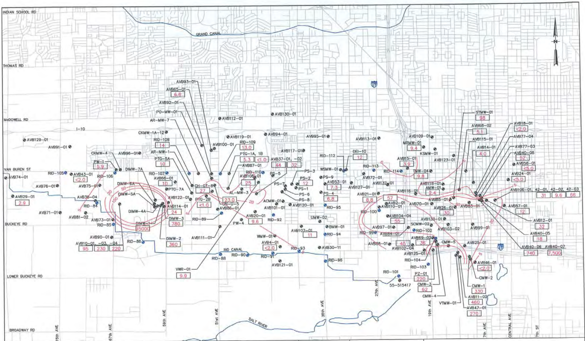
FIGURE 4-3 UAV 1 PCE CONCENTRATIONS-1998 WEST VAN BUREN WQARF SITE PHOENIX, ARIZONA
