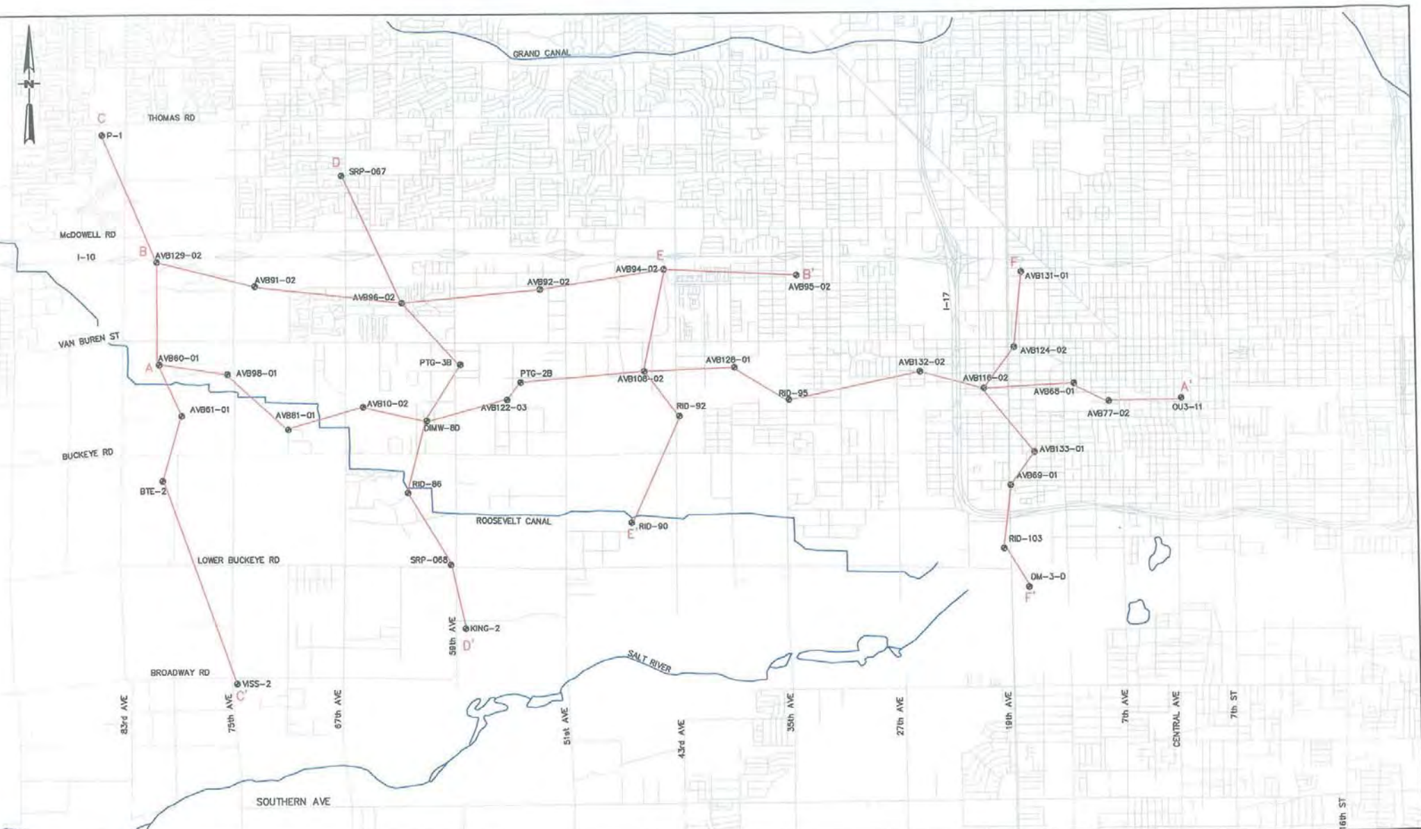
FIGURE 3-1 GEOLOGICAL CROSS-SECTION LOCATIONS WEST VAN BUREN WQRF SITE PHOENIX, ARIZONA
