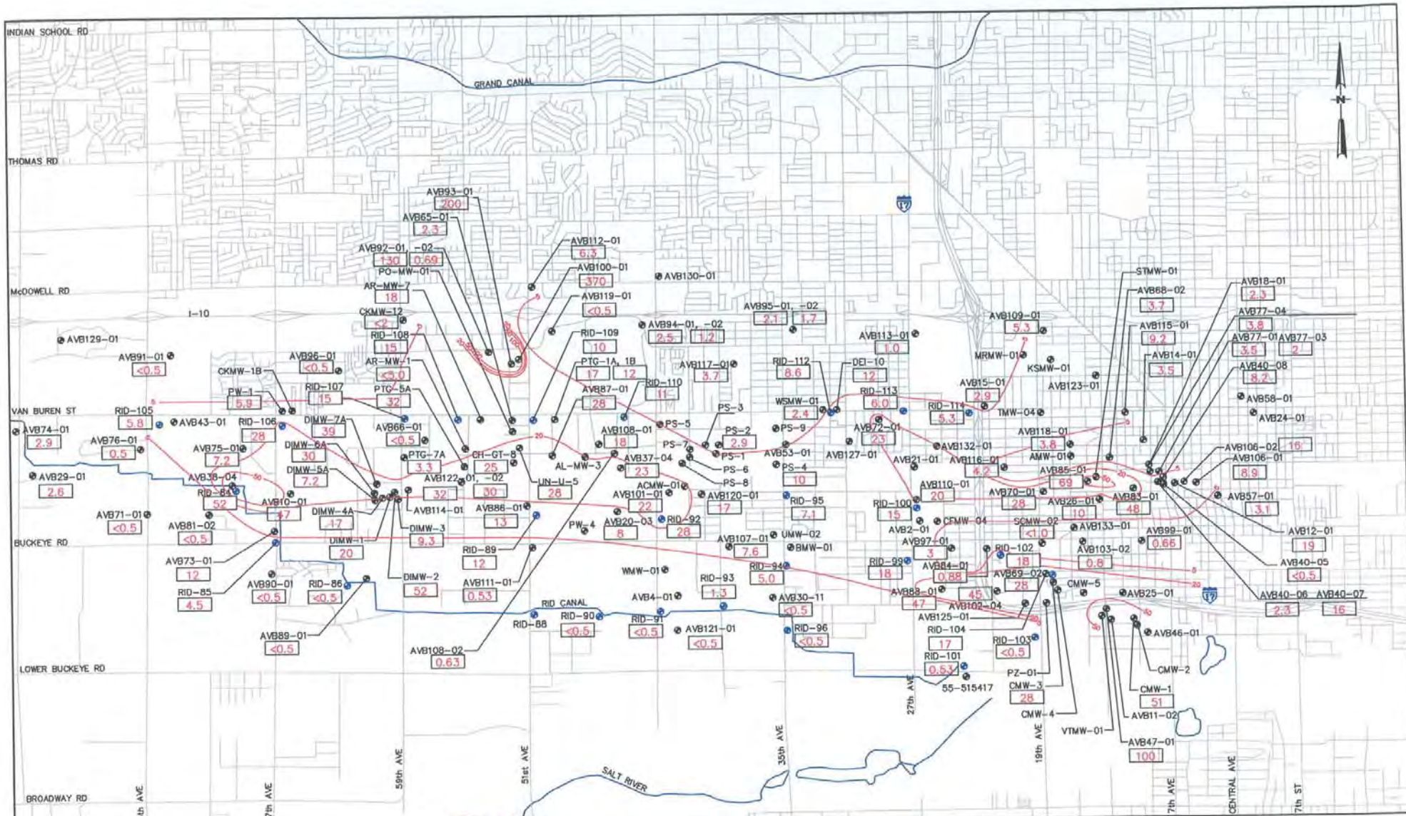
FIGURE 4-4 UAU 1 PCE CONCENTRATIONS-2003 WEST VAN BUREN WQARF SITE PHOENIX, ARIZONA
