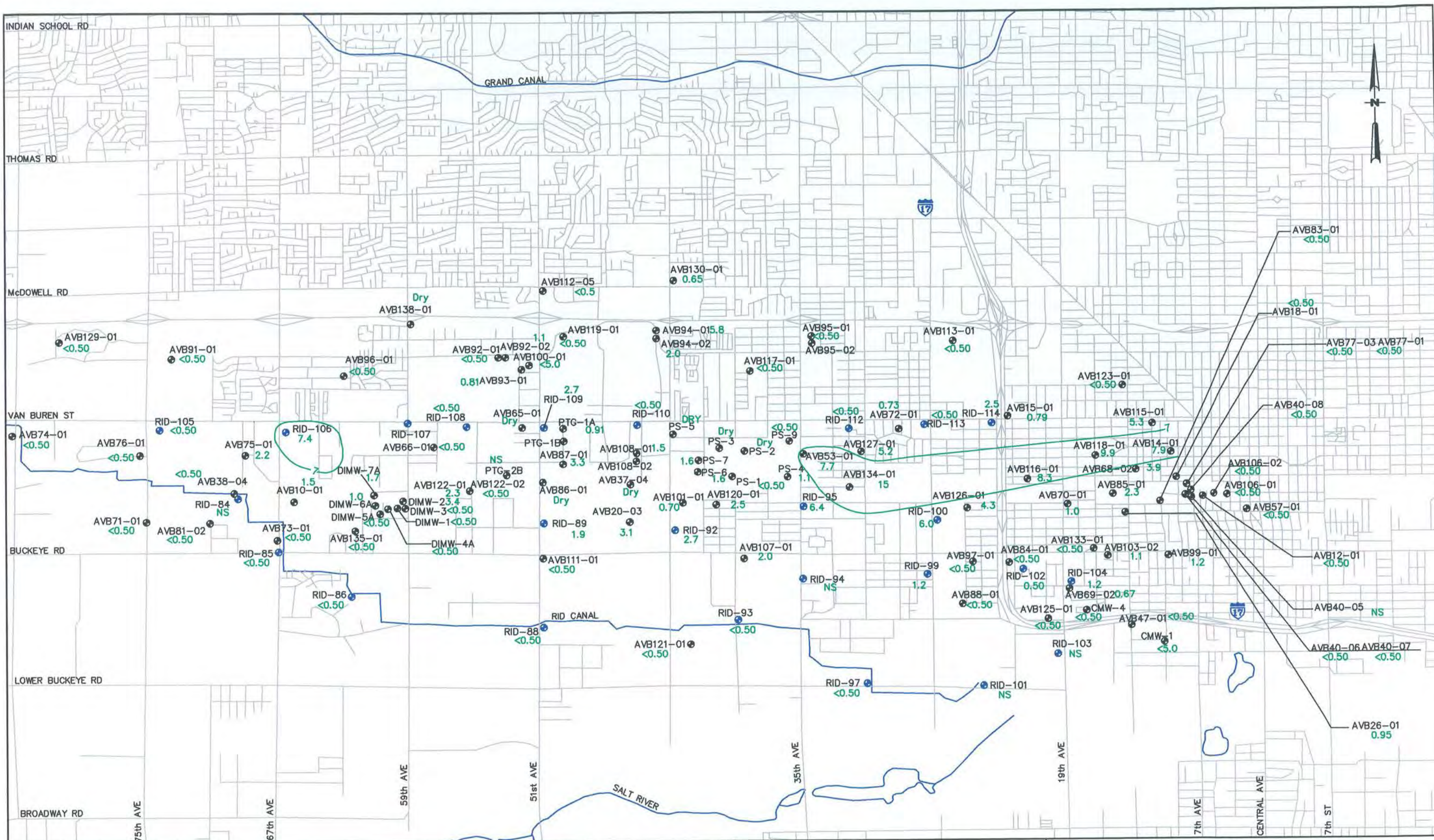
FIGURE 4-13 UAU 1 1,1 - DCE CONCENTRATIONS FIRST QUARTER 2008 WEST VAN BUREN AREA WQARF SITE PHOENIX, ARIZONA
