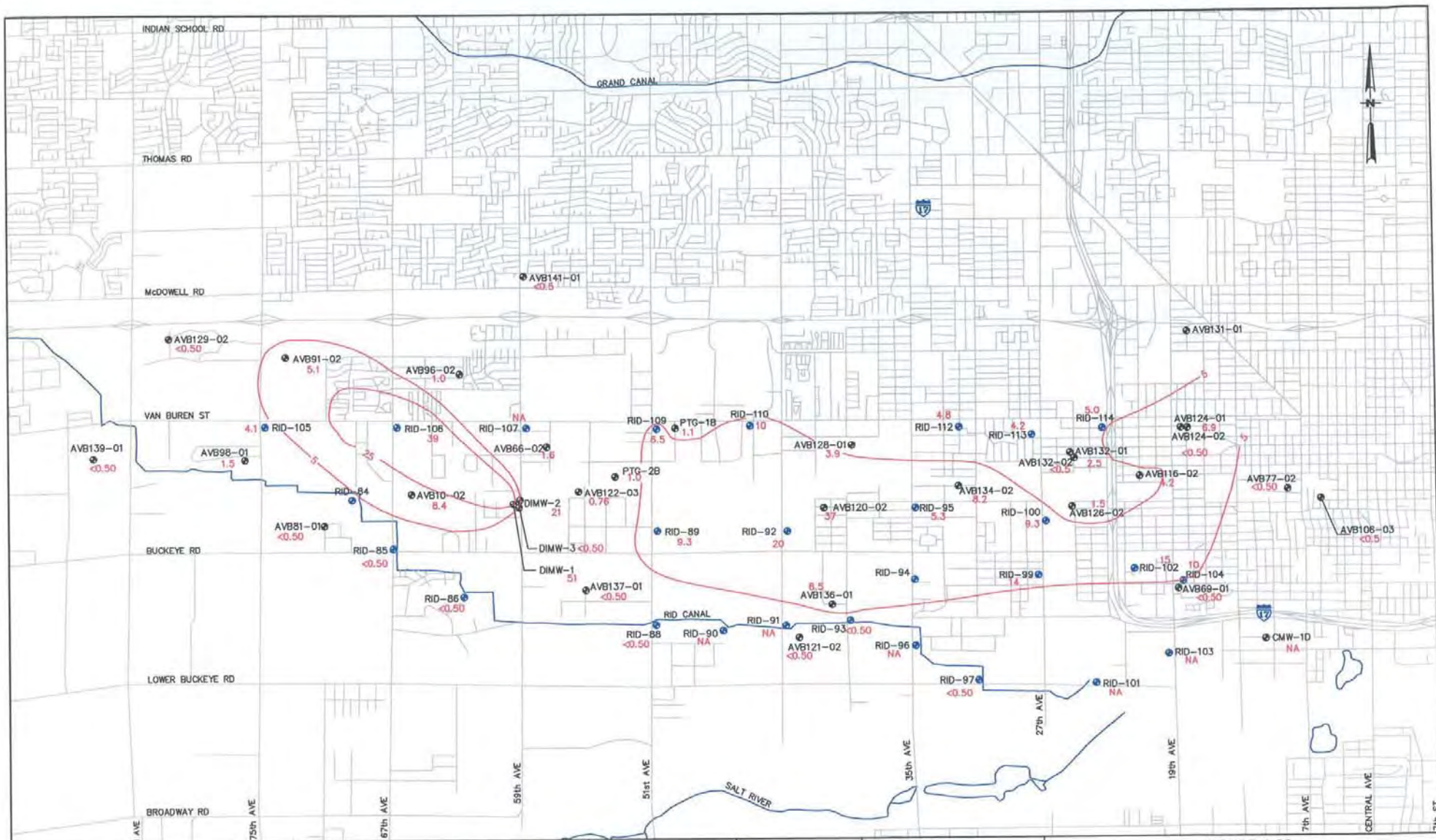
FIGURE 4-22 UAU 2 PCE CONCENTRATIONS FIRST QUARTER 2008 WEST VAN BUREN AREA WQARF SITE PHOENIX, ARIZONA
