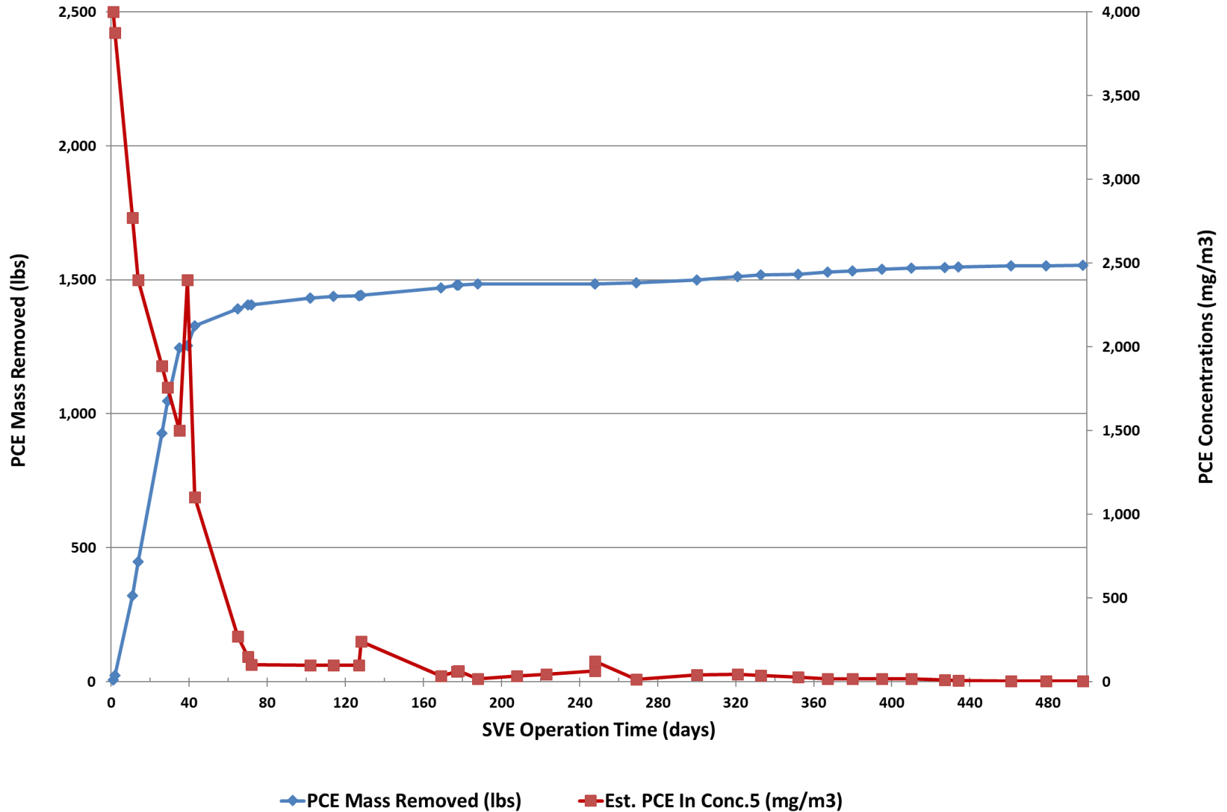
PCE Mass Removal and Concentrations vs. Time
