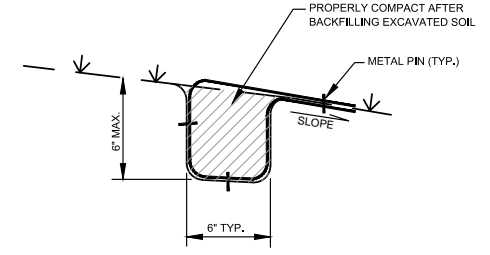
DETAIL D2 ANCHOR TRENCH NOT TO SCALE
