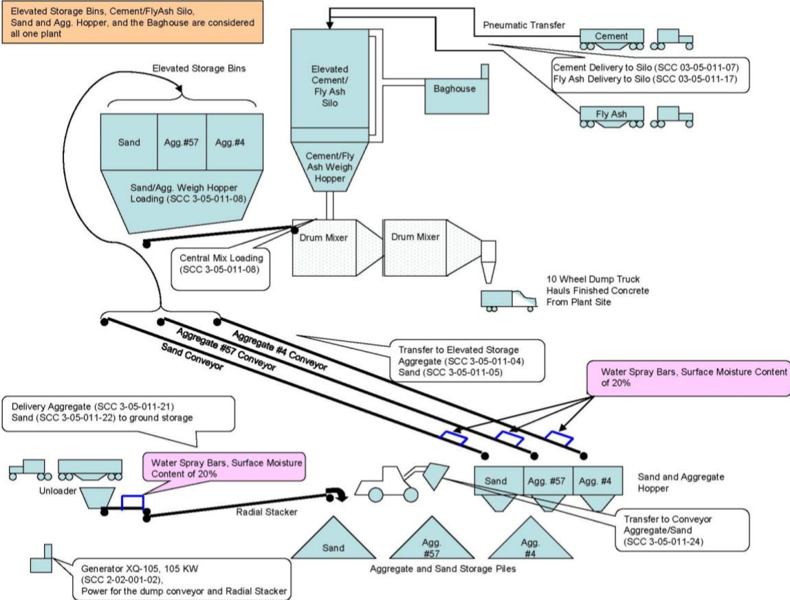
McNeil Brothers Inc.- Erie Strayer 2 Concrete Batch Plant Diagram
