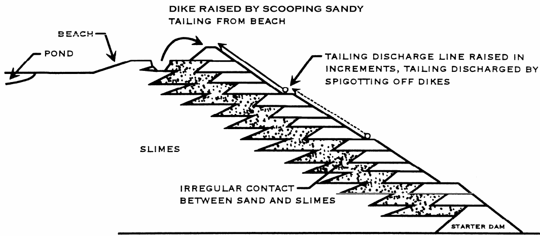
A. UPSTREAM METHOD OF TAILING DAM CONSTRUCTION
