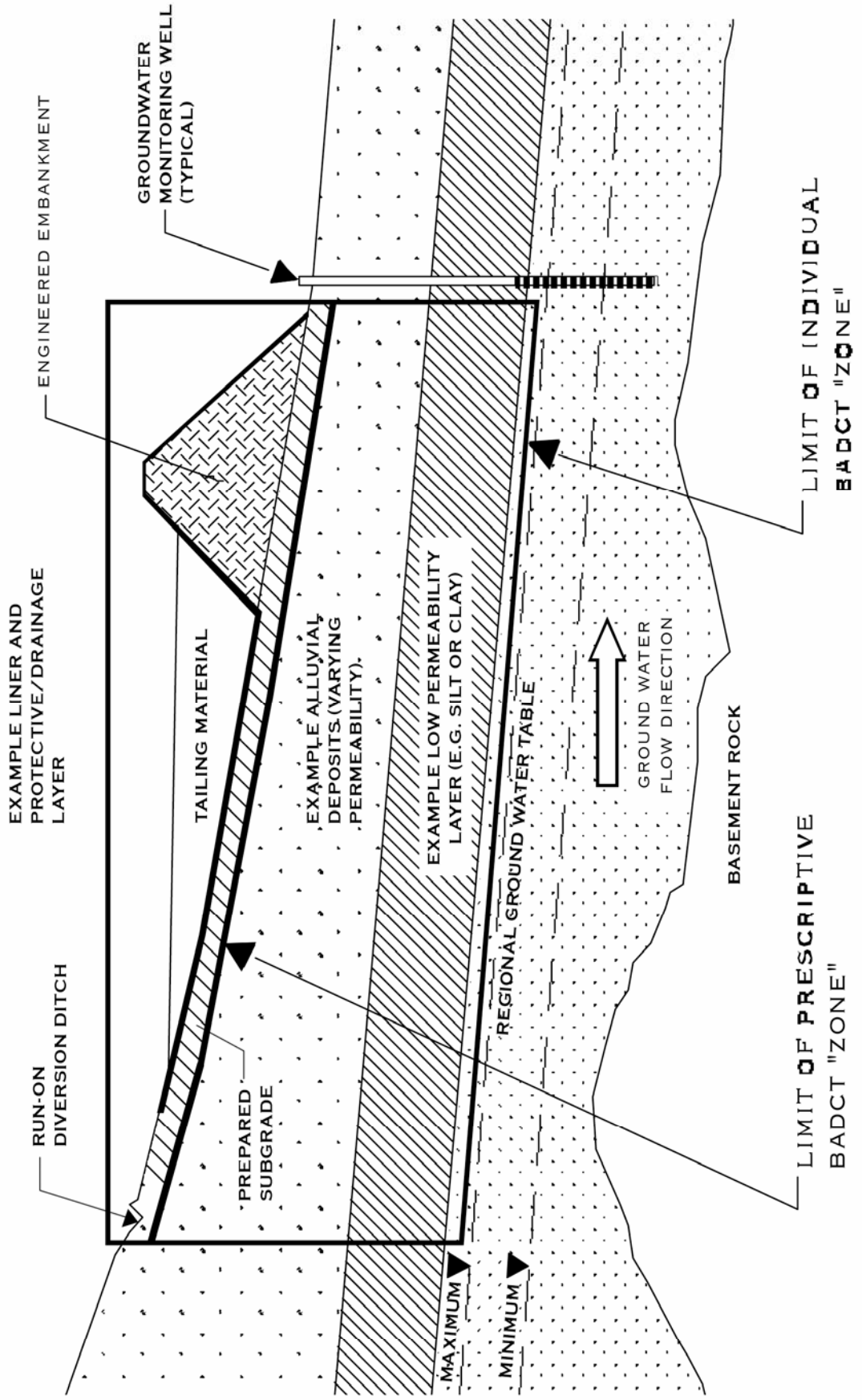
FIGURE 1-1 - EXAMPLE ILLUSTRATION OF PRESCRIPTIVE AND INDIVIDUAL BADCT "ZONES" (TAILING IMPOUNDMENT EXAMPLE)
