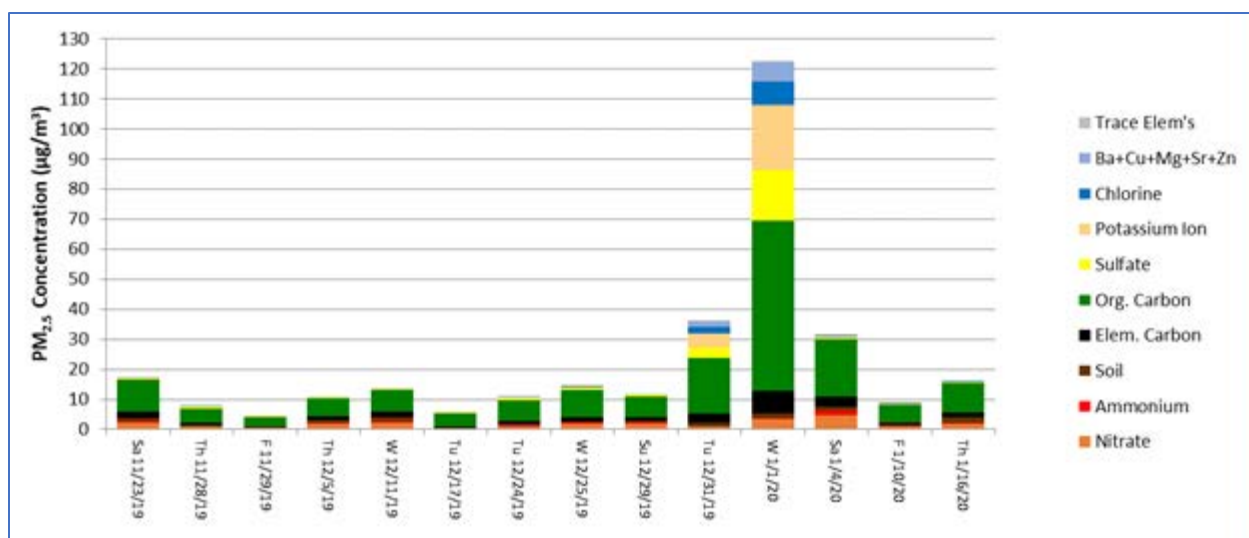
Figure 26 Chemical speciation samples collected at the West Phoenix site during the 2019-2020 study. The graph shows the total PM 2.5 concentration of the sample, as well as the concentration of chemicals within the samples. The IMPROVE algorithm is applied to the soil category.
