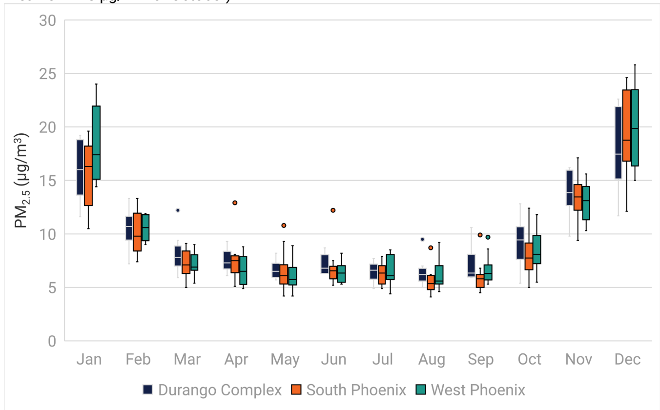
Figure 1. Interquartile range of monthly \text{PM}_{2.5} averages for the period 2014 - 2023 at the three violating monitors in Maricopa County. Note that the monthly mean only exceeds 9 \mu\text{g}/\text{m}^3 for the months November through February (Durango Complex is an exception with a monthly mean of 9.45 \mu\text{g}/\text{m}^3 for October).
