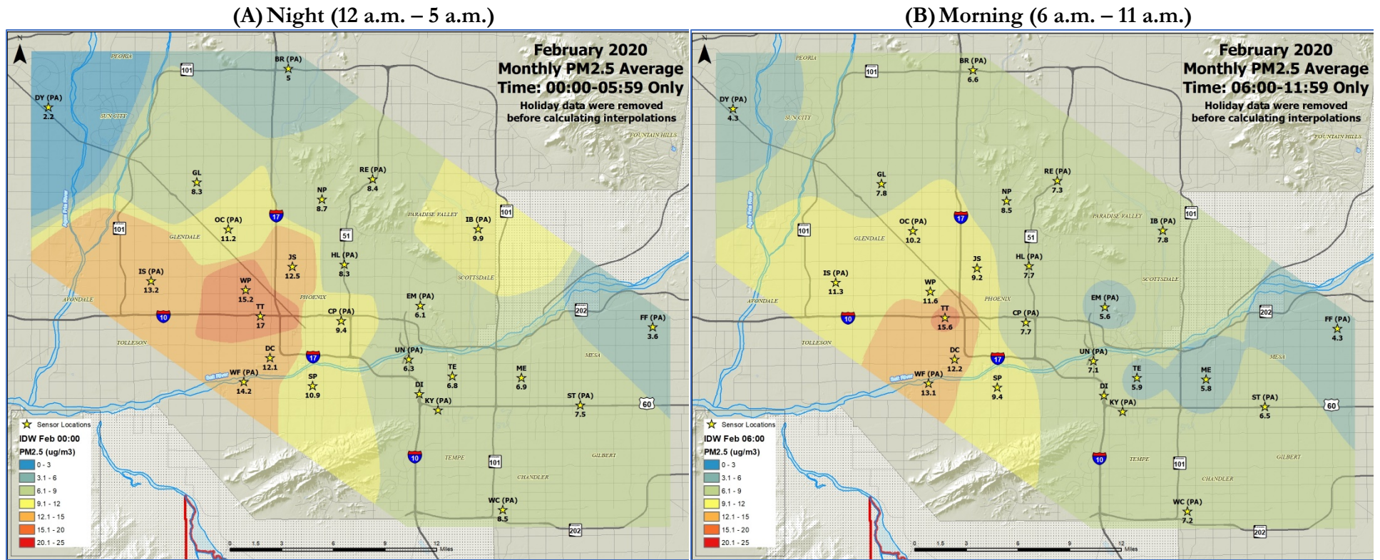
Figure 20. Spatial patterns of PM 2.5 for February 2020, averaged by time of day: Night (A), Morning (B), Afternoon (C), and Evening (D).
